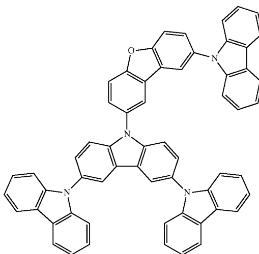
(Compound 15)
