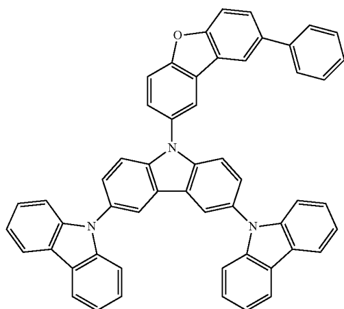
Compound (2)
